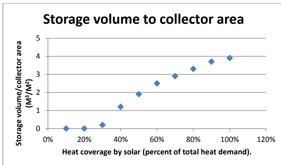
Figure 18 Ratio of seasonal storage volume to collector area (y-axis) as a function of solar heat coverage [4] and [5].
