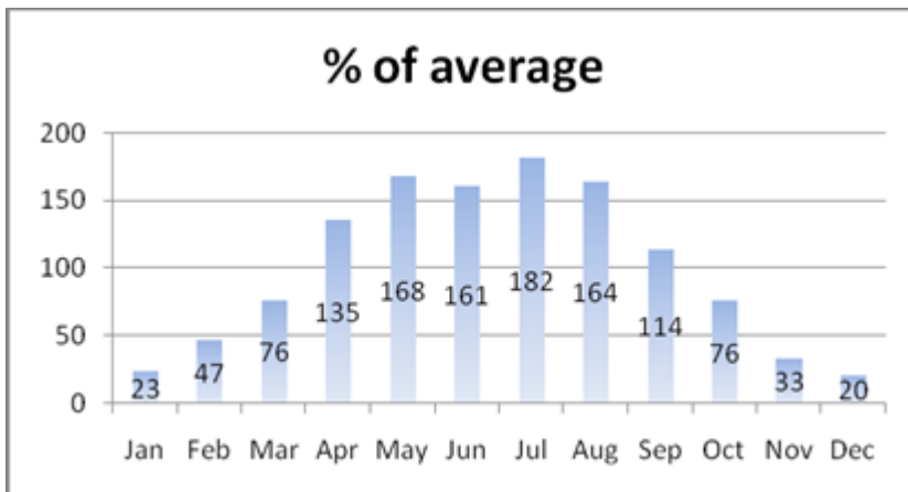
Figure 13 The seasonal variation of heat generation from typical solar collectors in Denmark [3].
