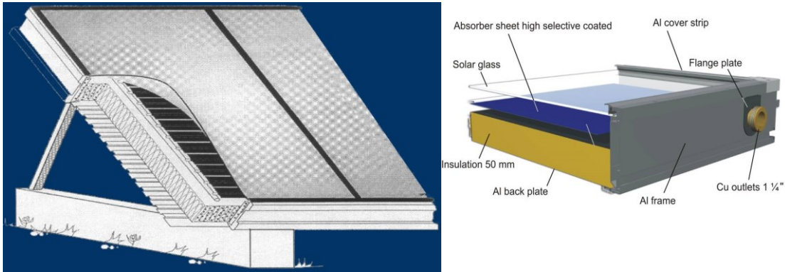
Figure 8 Basic principle of a flat plate solar collector.
