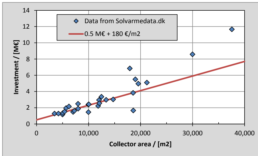
Figure 17 Solar plant investment for Danish SDH projects. The plant in the upper right corner is "Dronninglund" with 37,573 m 2 which includes a seasonal heat storage – and the investment for that is 2.4 M€ (see the section below on the seasonal heat storage), bringing this plant closer to the red line [5].
