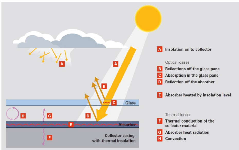
Figure 9 Example of utilisation rate of solar energy and effects influencing the efficiency. [10]
