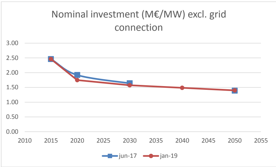
Figure 22 Expected cost development offshore 2019 compared to 2017.
