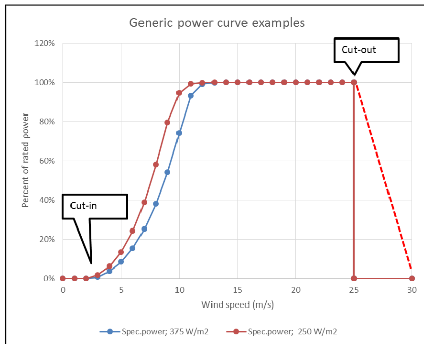
Figure 3 Turbine power curves (Information's from expert workshop held by DEA 27-4-2015). Specific power values refer to e.g. 3 MW with 124m rotor diameter (250 W/m 2 ) and 3 MW with 101 m rotor diameter (375 W/m 2 )
