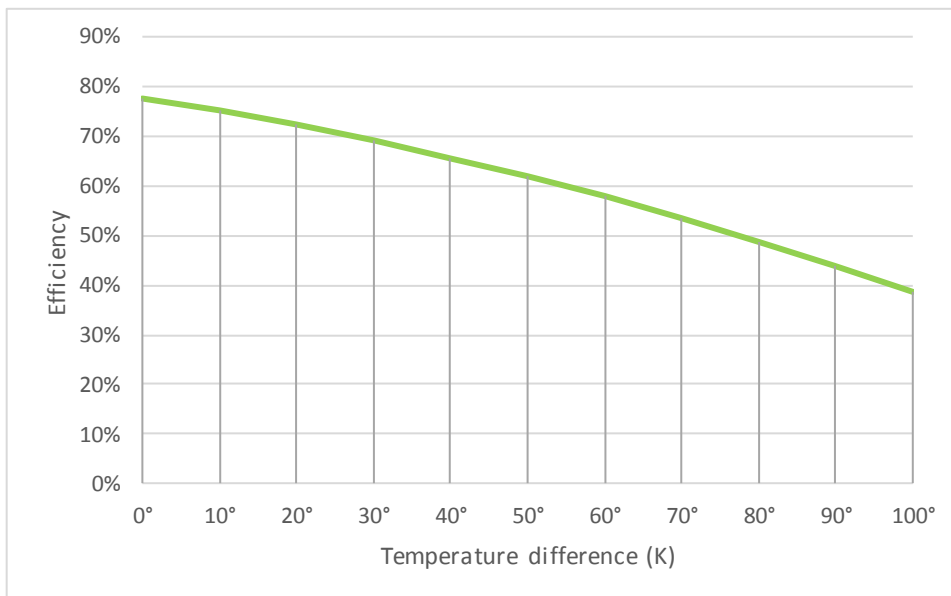
Figure 10 Efficiency as a function of temperature difference. (Based on data from [8], example with G=1.000 \text{ W/m}^2 , \eta_0=0.777 , a_1=2.41 , a_2=0.015 ) 20
