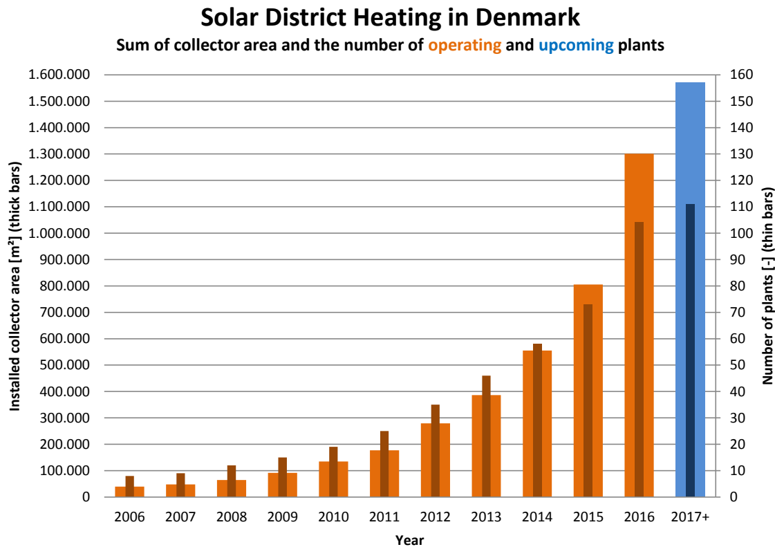
Figure 14 Solar district heating plants in Denmark in operation (until 2017) and planned. The trend is that the new plants are larger and include seasonal heat storages [5].
