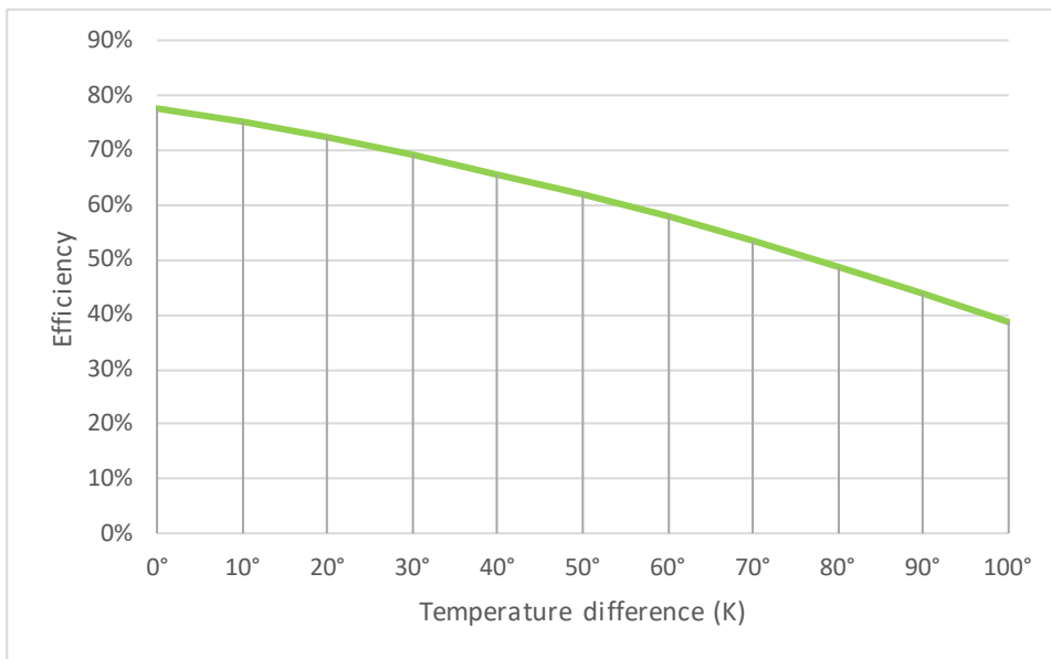
Figure 3 Efficiency as a function of temperature difference. (Based on data from [8], example with G=1.000 \text{ W/m}^2 , \eta_0=0.777 , a_1=2.41 , a_2=0.015 ) 28
