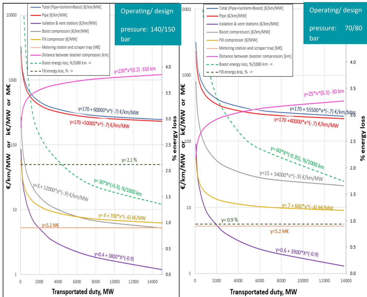
Figure 15: Estimated CAPEX, compression losses and distance between booster compressor vs. transported duty (HHV) for hydrogen transmission pipes. Examples of how to use the figures are given in tables below.
