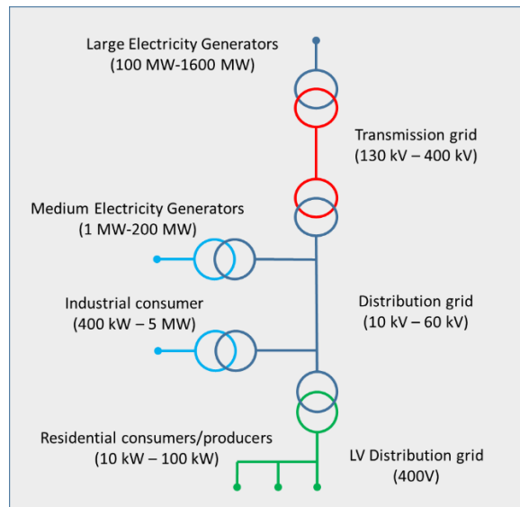
Figure 1: Major components in an electric power grid
