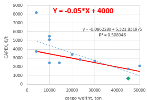
Figure 24: CAPEX of L20 ships (including CO 2 carrying ships) vs cargo weight from various obtained examples (green point is price for diesel tanker which is cheaper as no pressure or refrigerated vessels)
