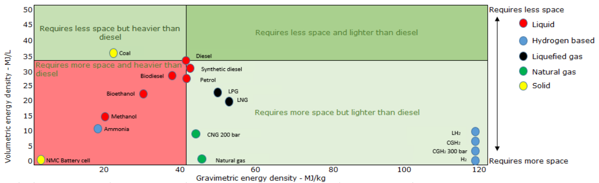
Figure 2: Energy density for various fuels
