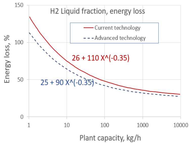
Figure 10: Energy loss associated with liquefaction of H 2 [ref.19]
