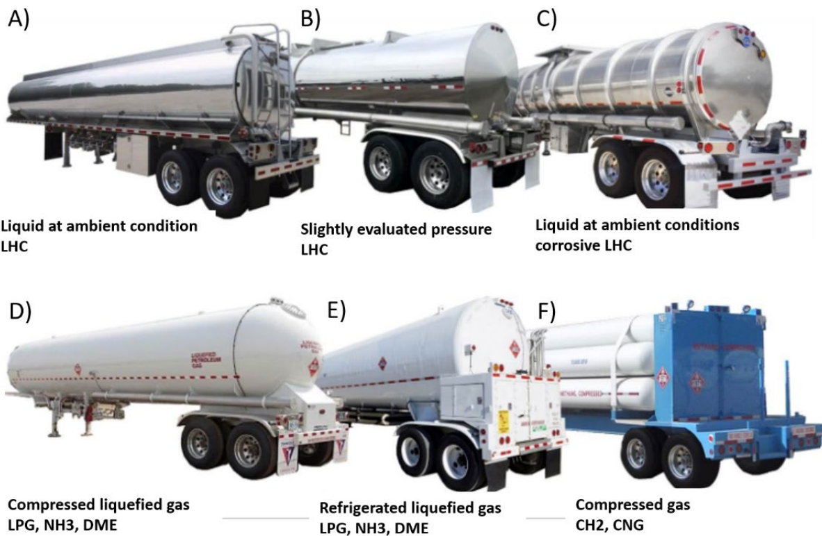
Figure 17: Different tank trailer design [ref. 22].
