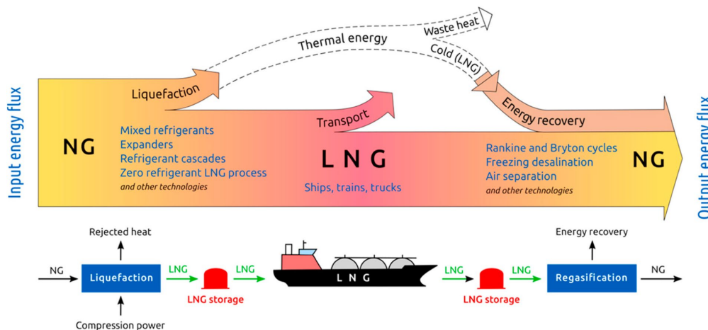
Figure 9: Illustration of steps and losses in transport of LNG. The other liquefied fuels include the same steps [ref. 11]
