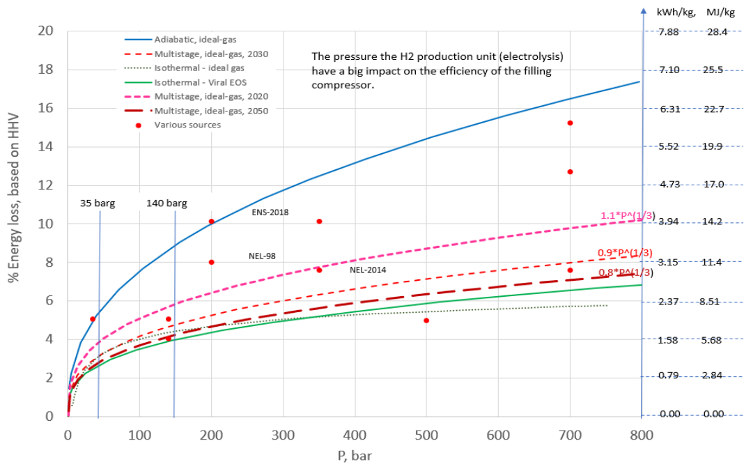
Figure 11: Energy loss for adiabatic, multistage with interstage cooling and isothermal compression (reciprocating H2 compressors). Points from various sources have been added. Numbers along the secondary y-axis are absolute loss.
