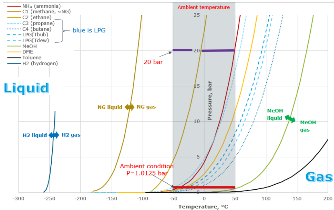
Figure 3: Phase curve for various fuels. Toluene is representative for LOHC which all are liquid at ambient condition. All hydrocarbon mixtures above C5 and all alcohols are below the MeOH curve
