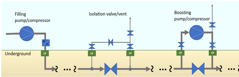
Figure 13: Major elements in a transmission pipe net
