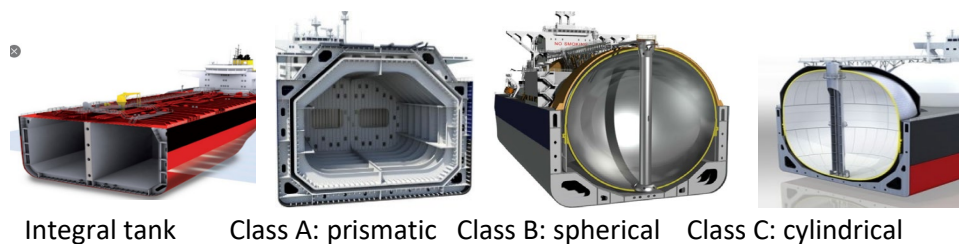
Figure 23: Different tank classes. The most cost-efficient onboard storage of ammonia seems to be class C (pressurized tanks) (Topsoe, 2020).
