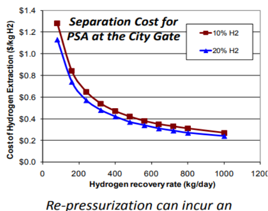
Figure 5: Separating H 2 from NG using PSA ref. 19
