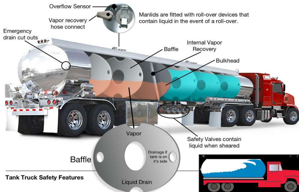
Figure 19: Tank safety features and internal baffles to prevent liquid splashing when driving.
