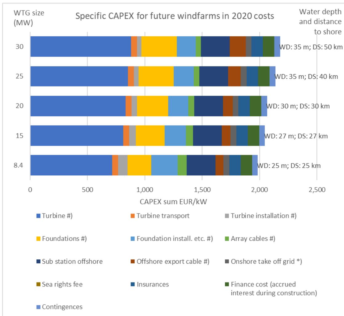
Figure 9 Detailed cost breakdown for future wind farms without learning rates.
