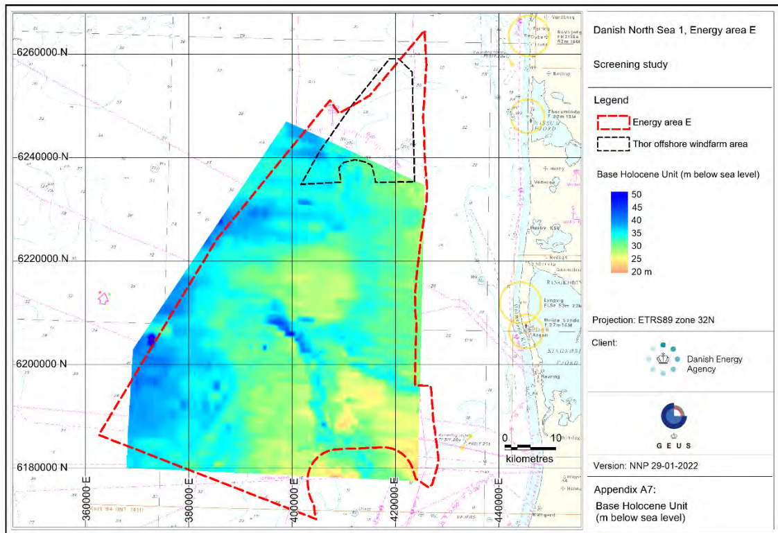
Figure 6-17. Mapped base of Holocene Unit (m below sea level). Corresponds to paleolandscapes before Holocene marine transgression. Appendix A7.
