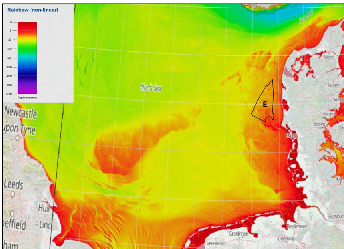
Figure 5-1 Bathymetrical map of the North Sea (From EMODnet). The black polygon shows the area E in the Danish North Sea.
