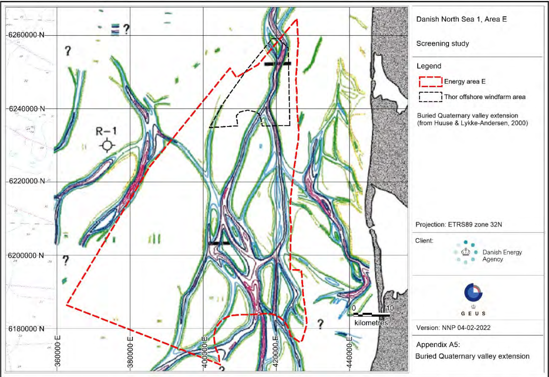
Figure 6-8. Mapped buried valley pattern in the screening area (modified from Huuse & Lykke-Andersen, 2000). Appendix A5.
